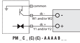
Switched DC
