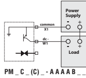
Open Collector
