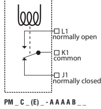
Mechanical Relay Form C
