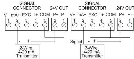
Transmitter Powered by Internal Supply (optional)
