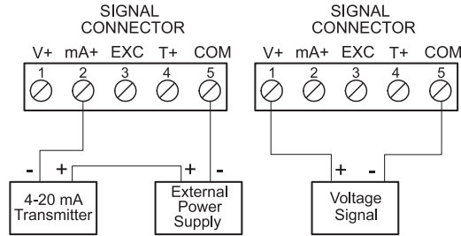
Transmitter Powered by External Supply
