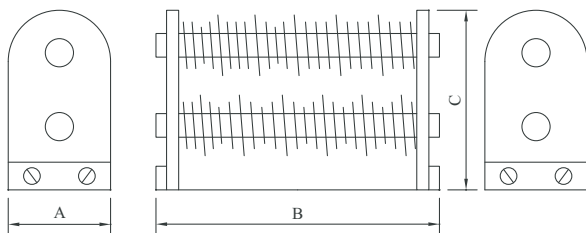
Dual Element Both Connections Same End Single Wattage
