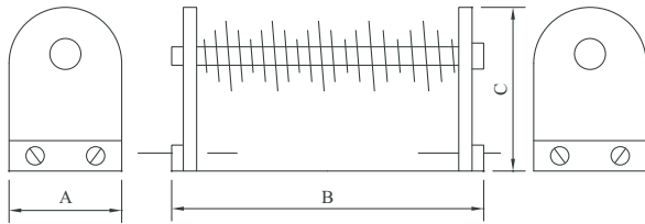
Single Element Both Connections Same End
