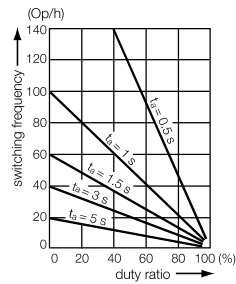
Intermittent periodic duty, ta: Motor starting time
