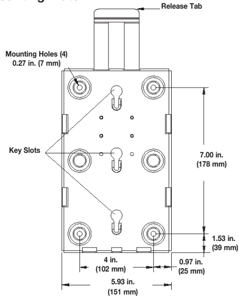
Mounting Plate
